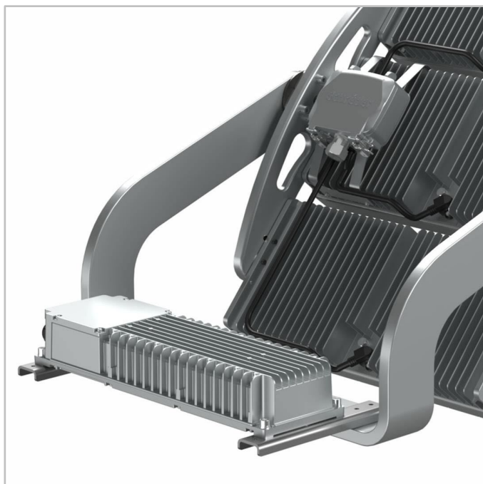
High-mast mounting fork (with integrated driver)
