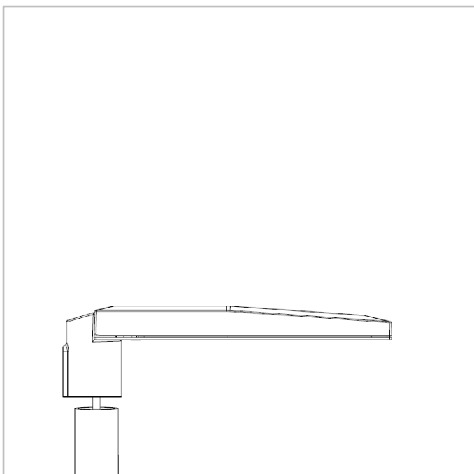
NIGHTSTAR | Post-top mounting for Ø76mm spigot - 2xM10 screws
