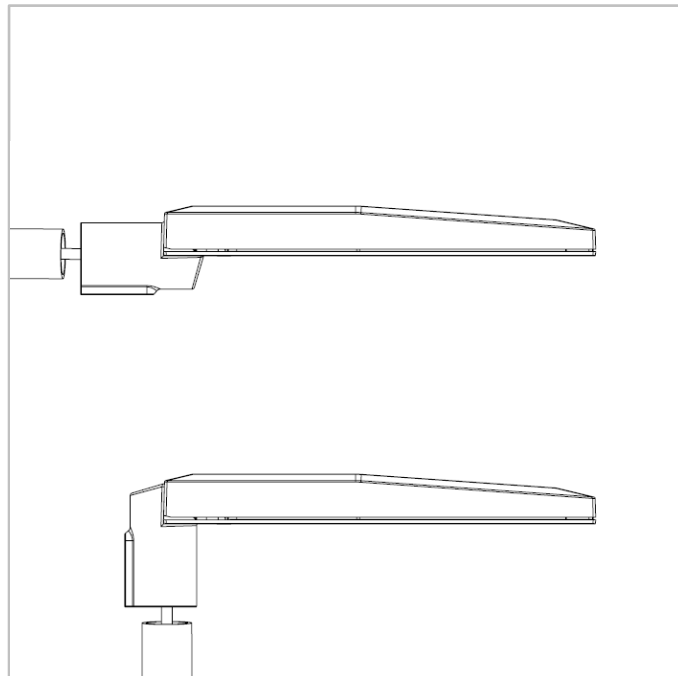
NIGHTSTAR | Side-entry or Post-top mounting for Ø60mm spigot - 2xM10 screws
